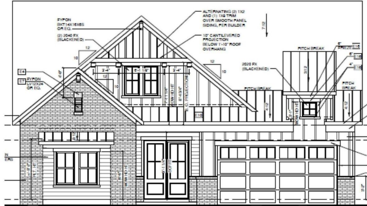
FRONT ELEVATION 'C' 1/4" = 1'-0" AT 20' X 34' LAYOUT 3/8" = 1'-0" AT 11' X 15' LAYOUT
